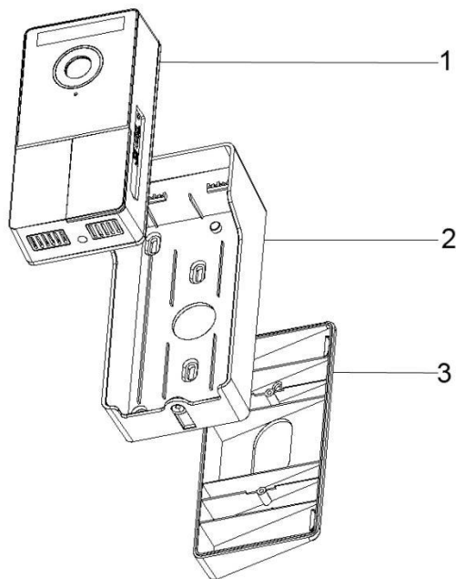
Figure 2-1 Appearance structure
