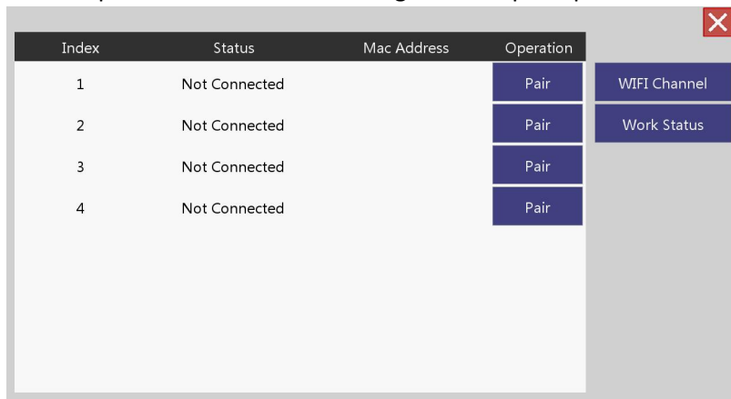
Figure 5-1 Add IPC
